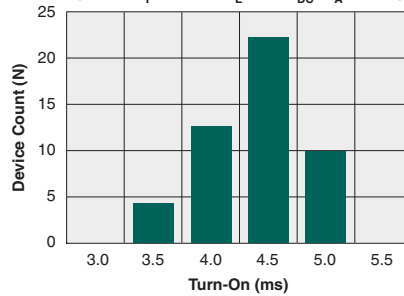
Typical Turn-On Time ( N=50, I_F=10\text{mA}, I_L=5\text{mA}_{\text{DC}}, T_A=25^\circ\text{C} )
