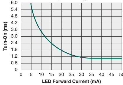
Typical Turn-On vs. LED Forward Current ( I_L=100\text{mA}_{\text{DC}} )
