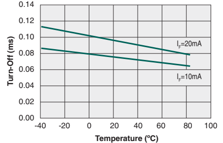
Typical Turn-Off vs. Temperature ( I_L=100\text{mA}_{\text{DC}} )
