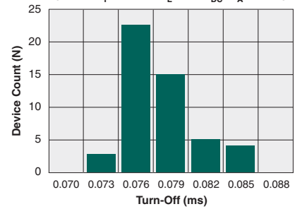
Typical Turn-Off Time ( N=50, I_F=10\text{mA}, I_L=5\text{mA}_{\text{DC}}, T_A=25^\circ\text{C} )
