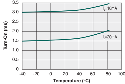
Typical Turn-On vs. Temperature ( I_L=100\text{mA}_{\text{DC}} )
