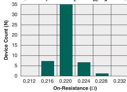
Typical On-Resistance Distribution ( N=50, I_F=10\text{mA}, I_L=1.0\text{A}_{\text{DC}}, T_A=25^\circ\text{C} )
